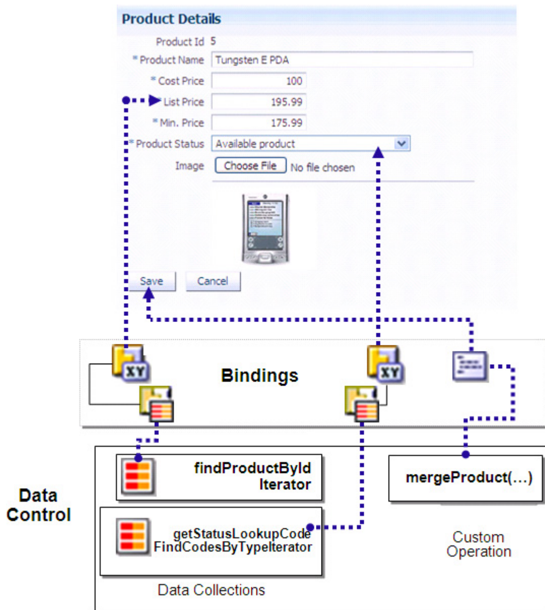
Figure 2–1 ADF Bindings
