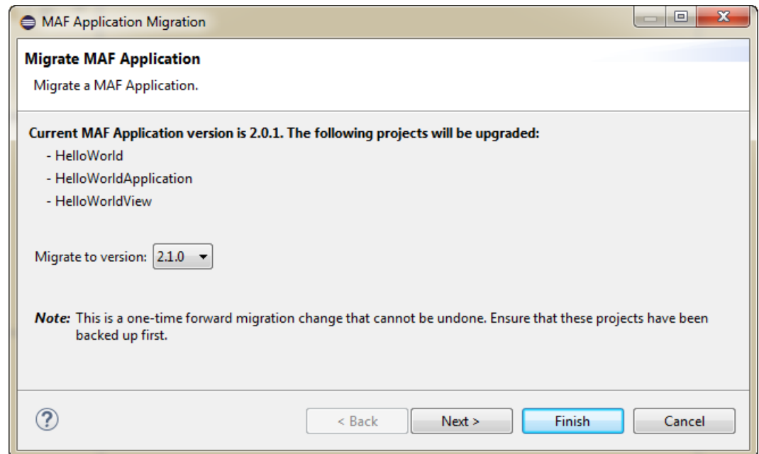
Figure 3–1 Migration Wizard
