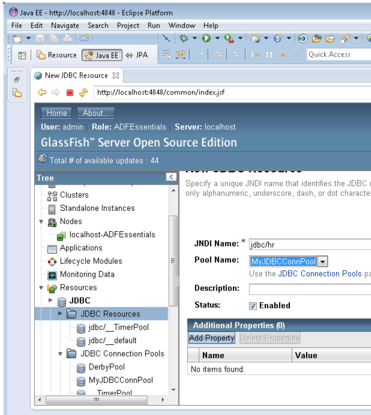
Figure 2-27 GlassFish Server Console - New JDBC Resource
