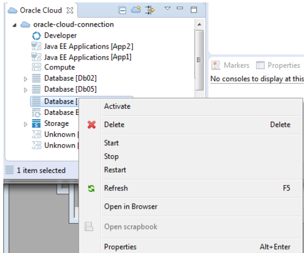
Figure 5-20 Activating Database as a Service
