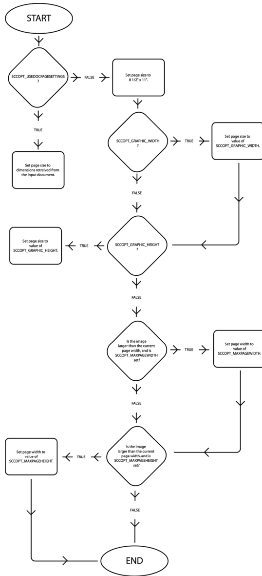
Figure 1 Logic Flow for Determining the Page Size of Spreadsheet and Database Pages
