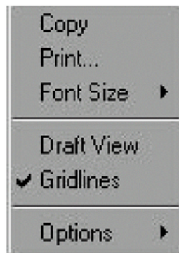
Figure 1 Context Menu
