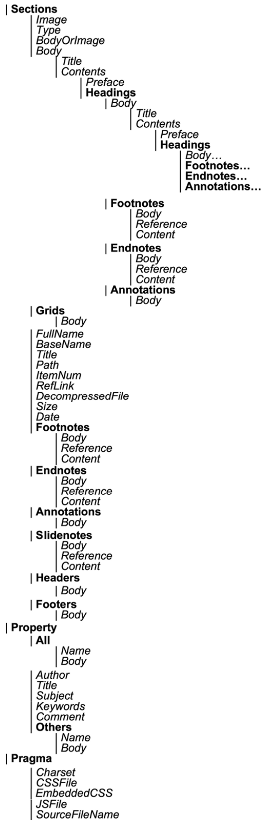
Figure 3-1 The Document Tree
