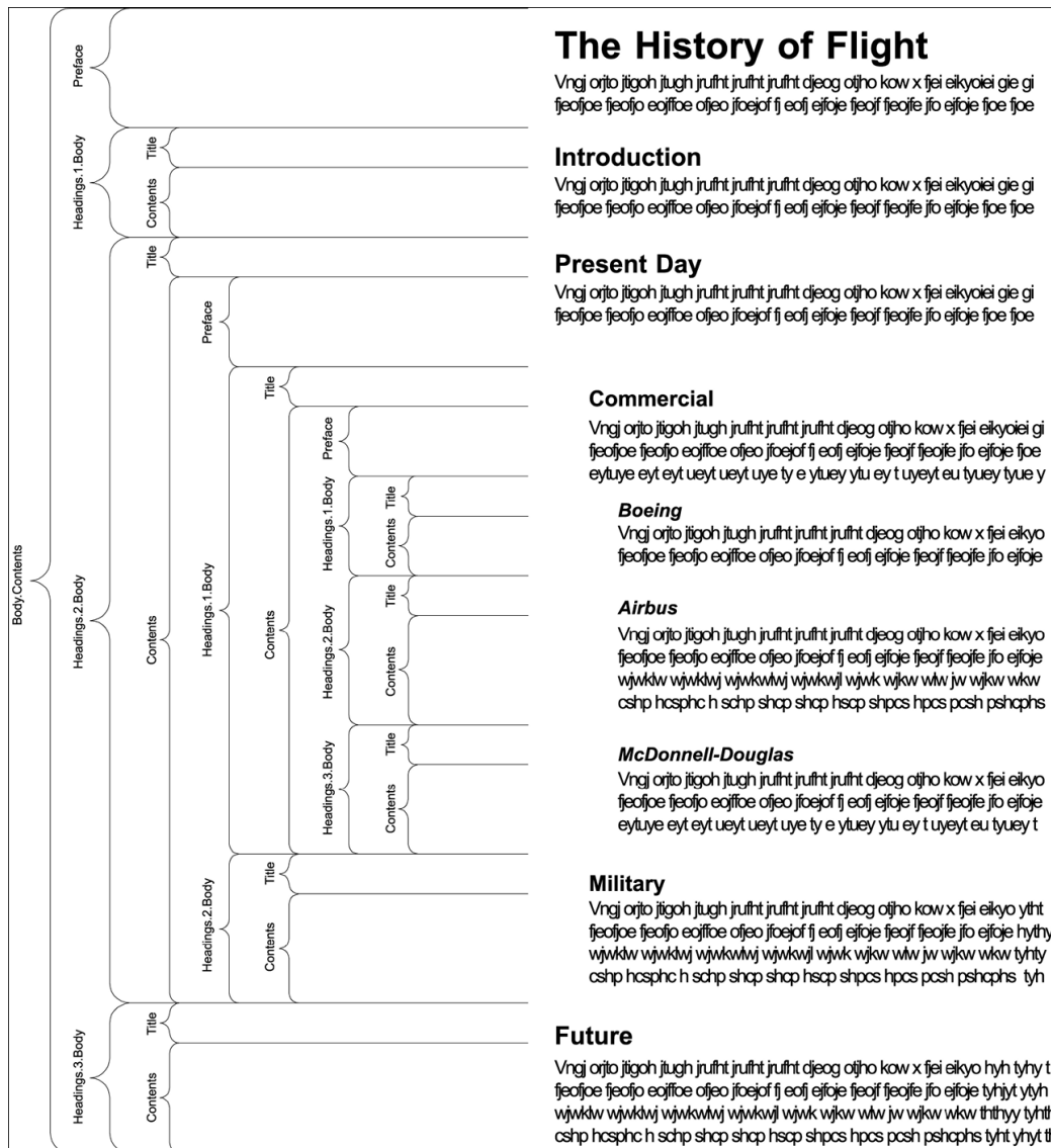
Figure 3-2 Correlation between Element Tree and Document
