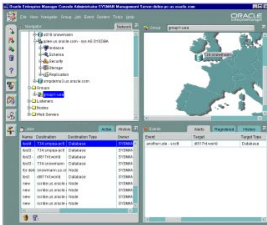
Figure 1-5 Oracle Enterprise Manager Console
