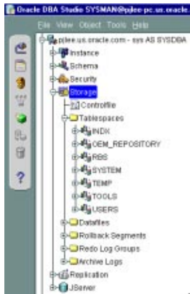
Figure 4–8 Managing Database Storage Parameters
