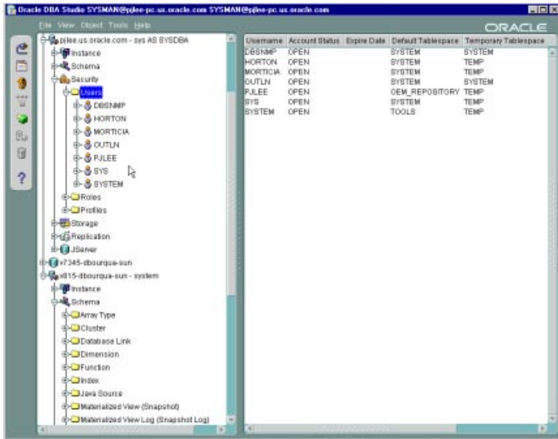
Figure 4–6 Security Management Window
