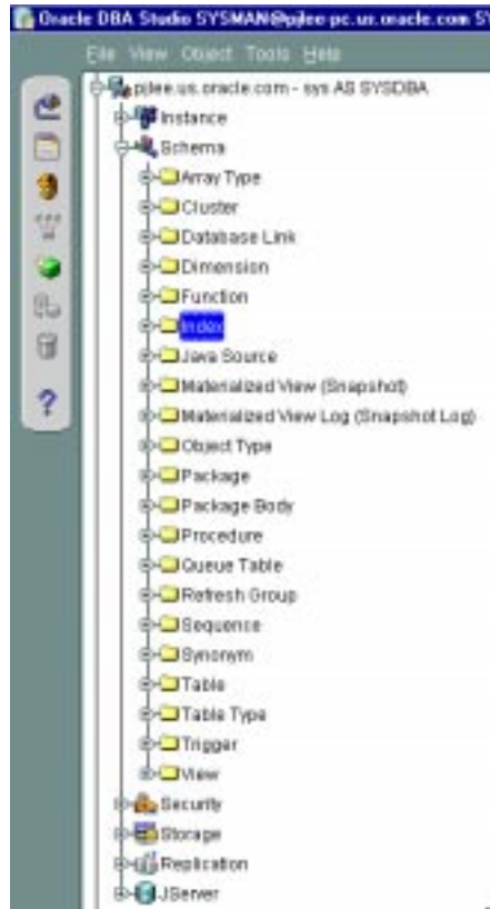
Figure 4–4 Schema Objects
