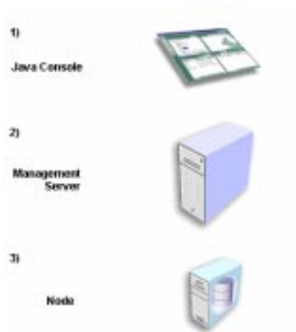
Figure 1–1 Three-Tier Architecture
