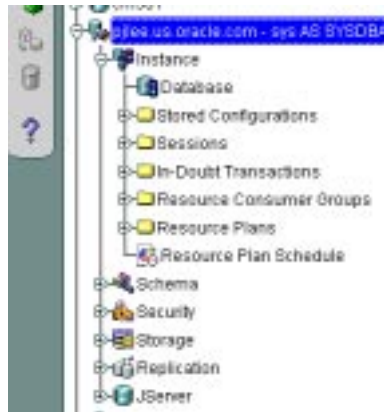
Figure 4–1 Instance Management Tree
