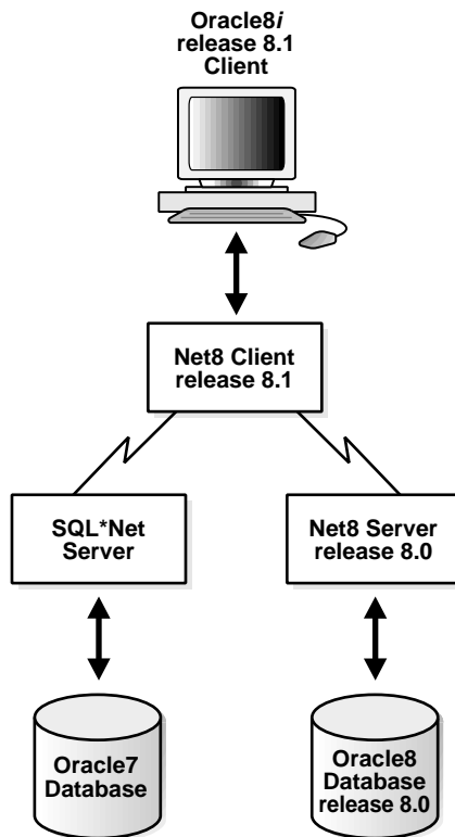
Figure F-3 Oracle8i Client to Oracle8 or Oracle7 Database
