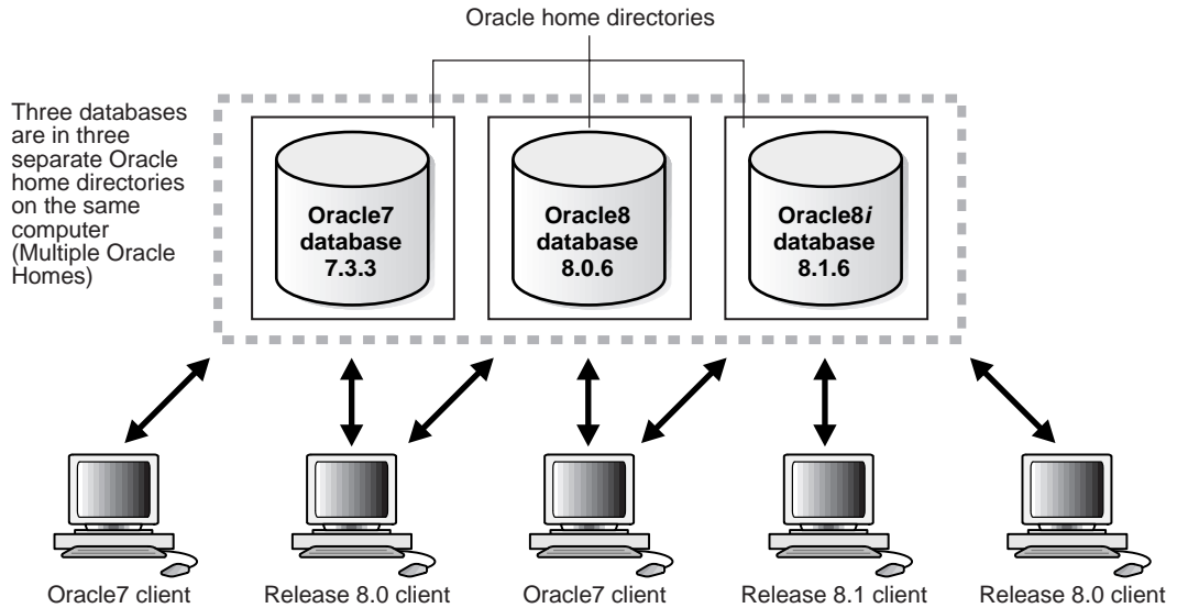
Figure 1-2 Version 7 and Version 8 Databases in Multiple Oracle Homes
