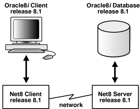
Figure F-1 Oracle8 Client to Oracle8i Database
