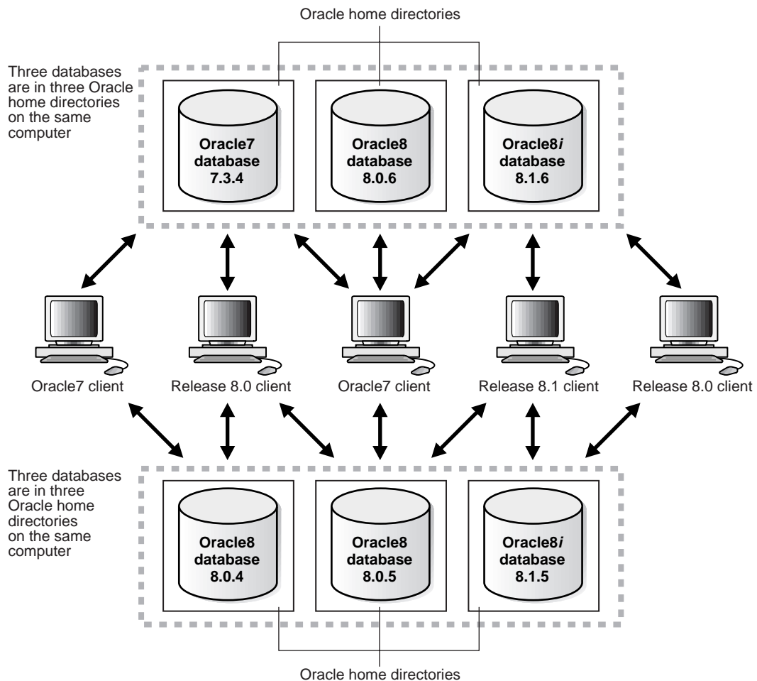
Figure 1-3 Version 7 and Version 8 Databases on Separate Computers
