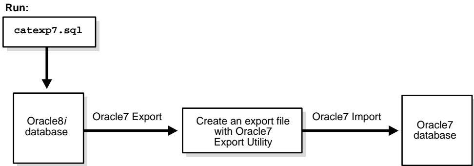
Figure 14-1 Downgrading to Oracle7
