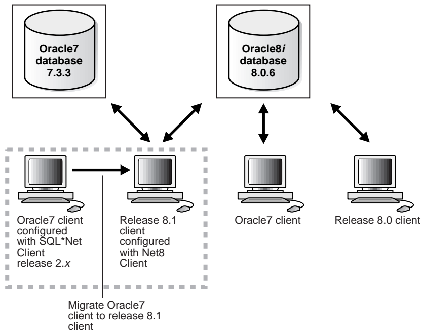
Figure 1-7 Migrate Version 7 Clients to Version 8 Clients
