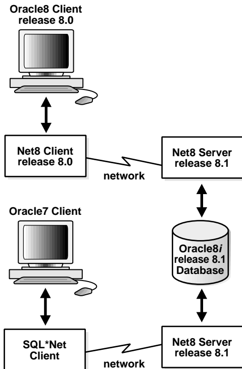
Figure F-2 Oracle8 Client release 8.0/Oracle7 Client to Oracle8i Database
