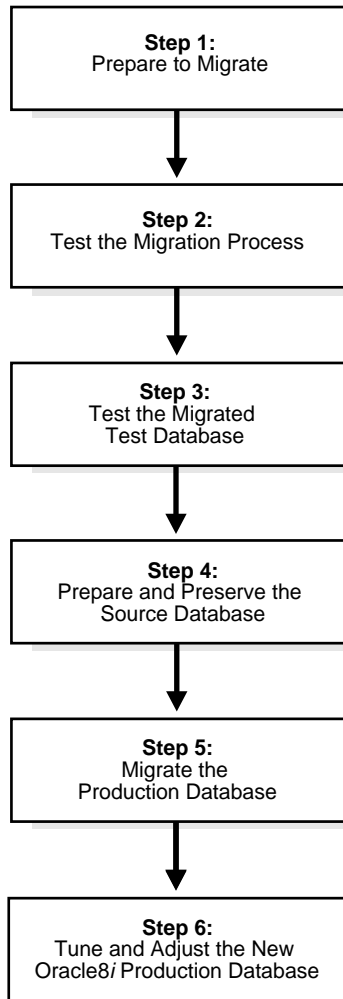
Figure 2–1 Major Migration Steps
