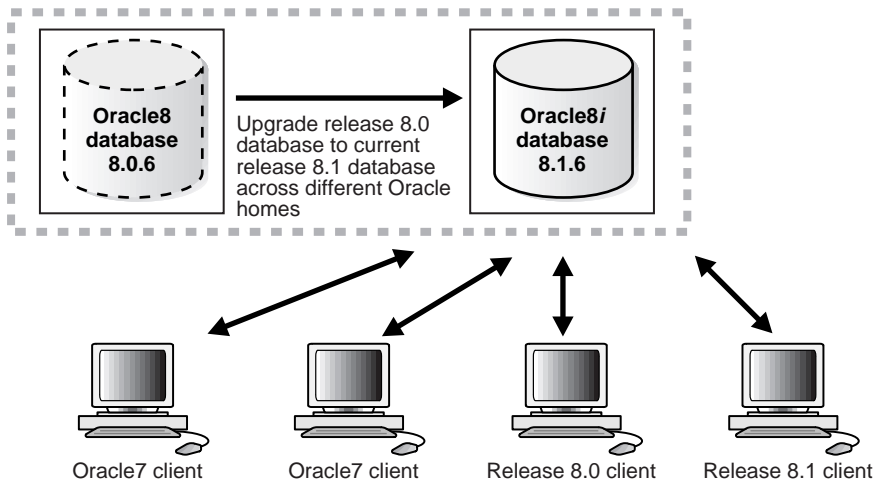
Figure 1-5 Upgrade a Release 8.0 Database to Release 8.1
